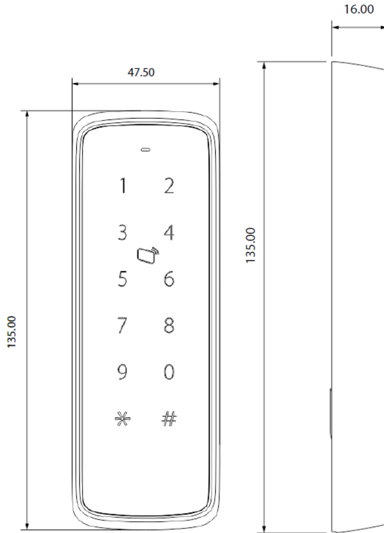
Figure 1-3 Dimensions (unit: mm[inch])
