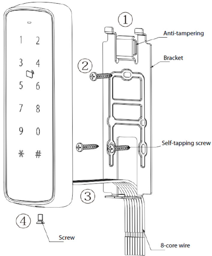
Figure 2-1 Installation process
